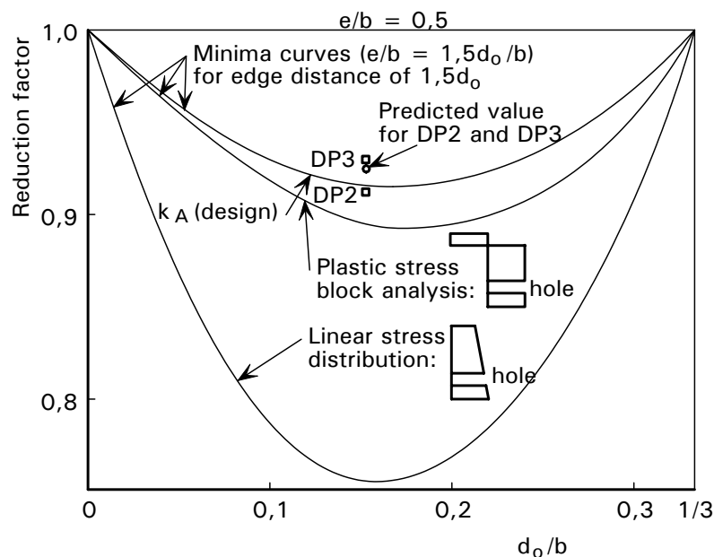
Figure C.4.9 Minima curves for k_A for holes at the edge distance of 1,5d_0
