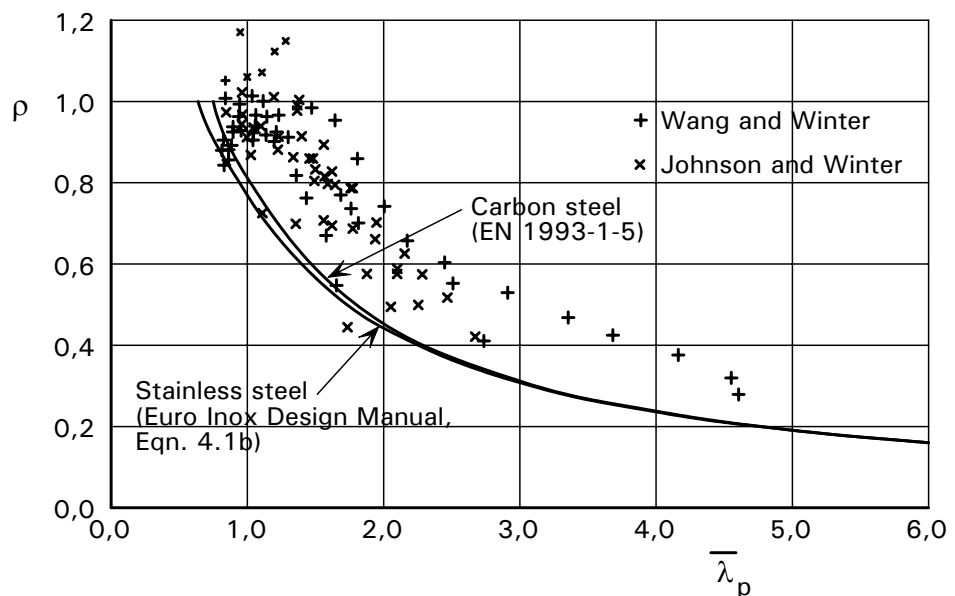
Figure C.4.3 Reduction factor versus plate slenderness for cold formed outstand elements
