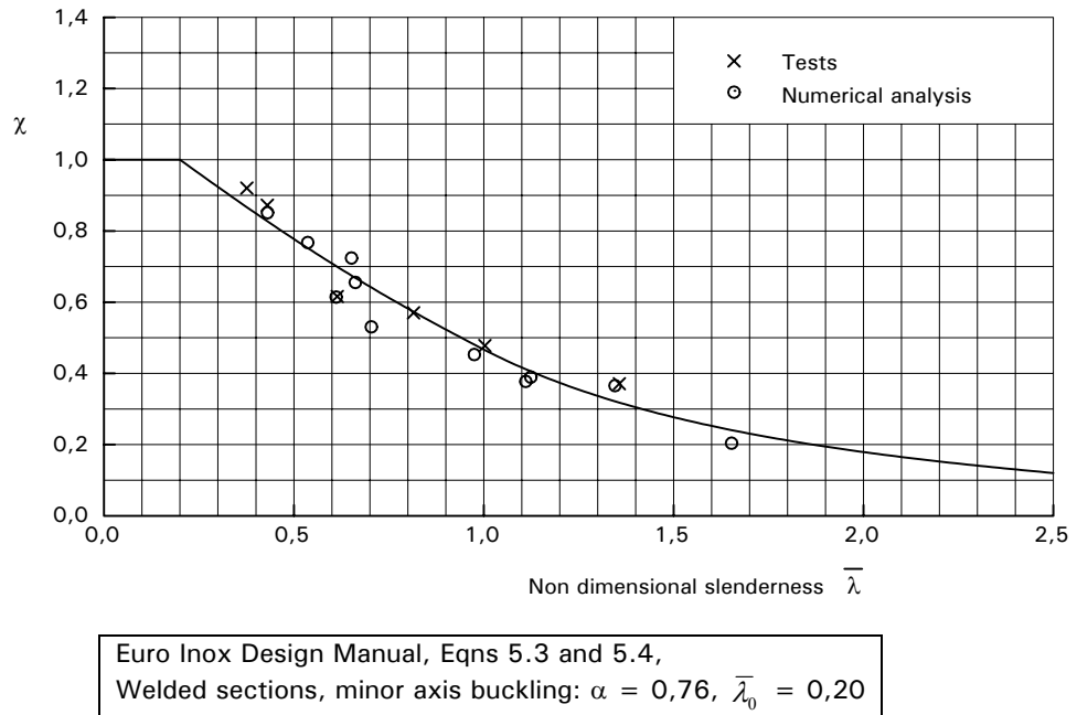
Figure C.5.10 Reduction factor versus non-dimensional slenderness for welded columns buckling about the minor axis
