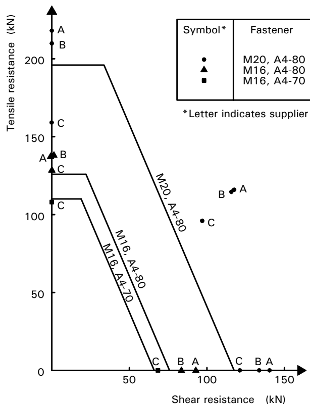
Figure C.6.7 Results of tests on stainless steel bolts
