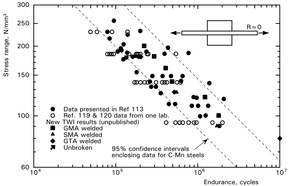
Figure C.8.3 Fatigue test results for austenitic stainless steel plates with longitudinal fillet welded attachments 117
