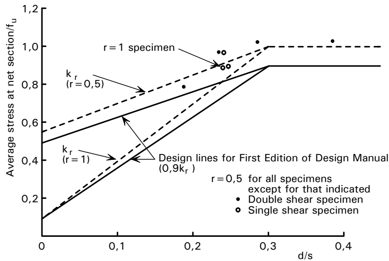
Figure C.6.6 Net section failure data by van der Merwe 99
