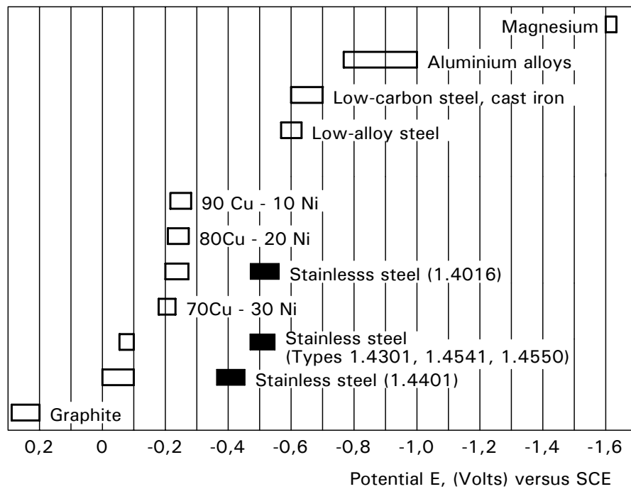
Figure C.3.10 Corrosion potentials of various materials in flowing seawater; potentials are measured against saturated calomel electrode (SCE). The black bars indicate potential in low velocity or poorly aerated water and in shielded areas
