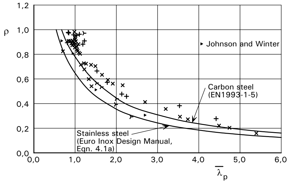
Figure C.4.2 Reduction factor versus plate slenderness for cold formed internal elements
