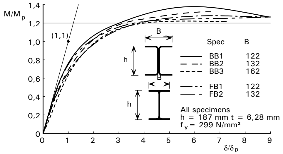
Figure C.4.10 Moment/deflection response of tested beams
