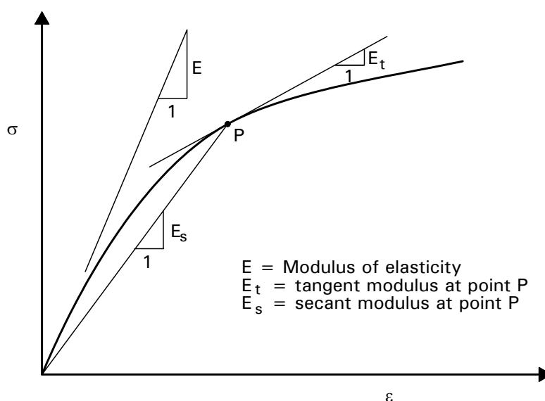
Figure C.5.15 Young's tangent and secant moduli
