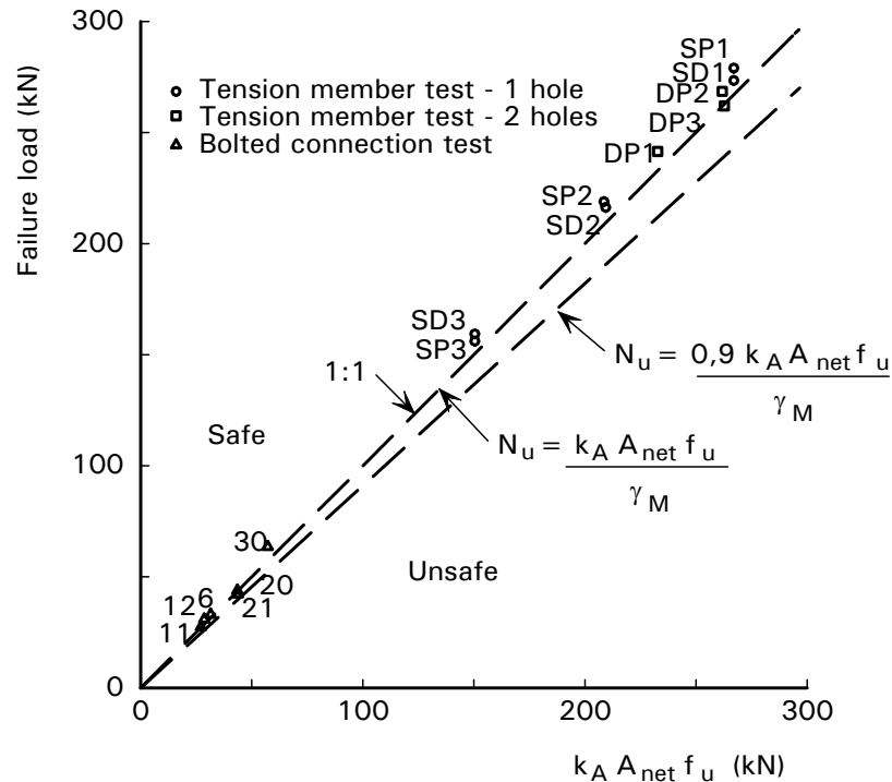
Figure C.4.7 Net section failure data ( \gamma_M = 1,0 )
