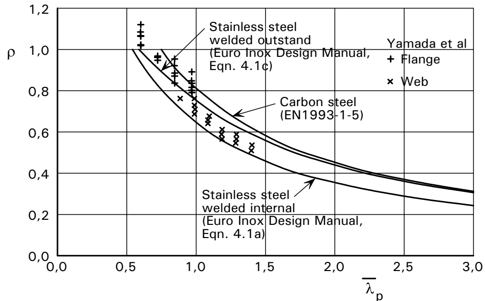
Figure C.4.4 Reduction factor versus plate slenderness for welded elements
