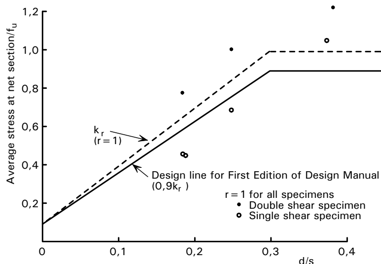
Figure C.6.5 Cornell University data for net section failure 17
