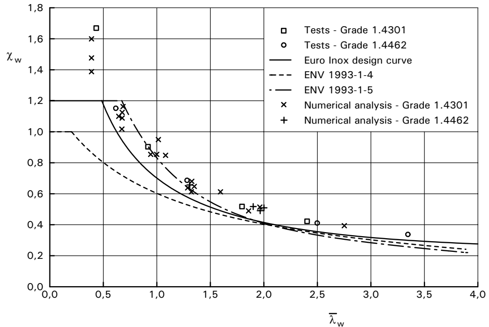
Figure C.5.13 Reduction factor versus non-dimensional slenderness for shear buckling of webs
