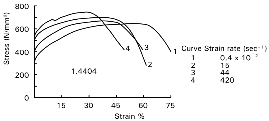
Figure C.3.6 Strain rate effects on grades 1.4307 and 1.4404
