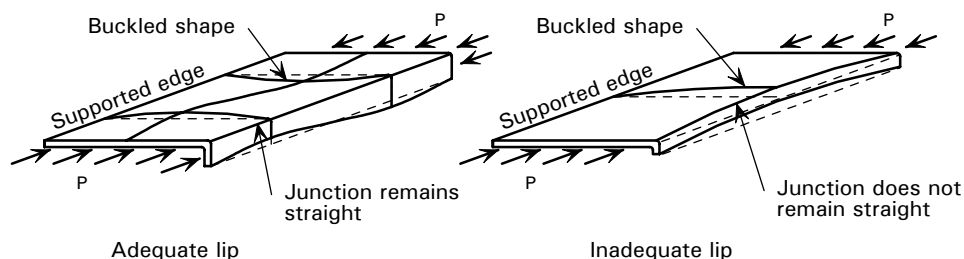
Figure C.4.6 Adequate and inadequate lips
