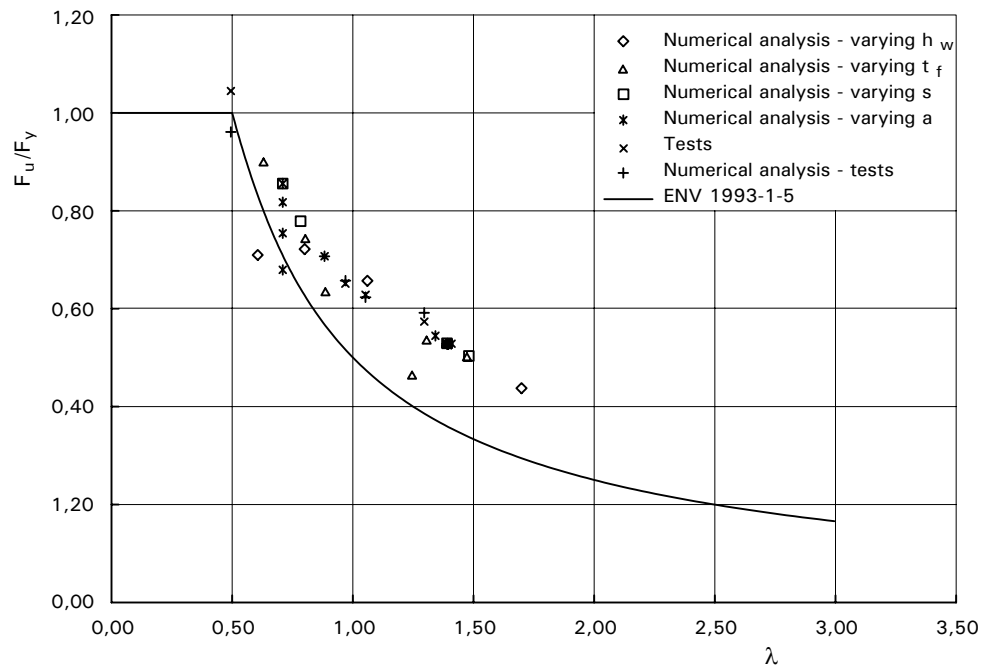
Figure C.5.14 Web crippling of stainless steel beams – test data and design curve
