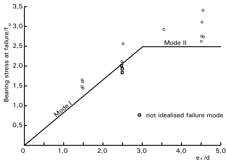
Figure C.6.4 Comparison of experimental data from Cornell University data with design lines 17
