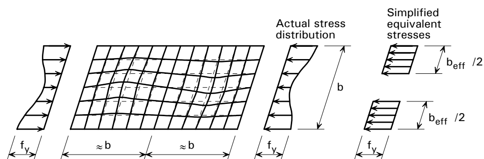
Figure C.4.1 The effective width concept
