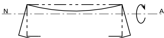
Figure C.4.5 Deformations in flange curling
