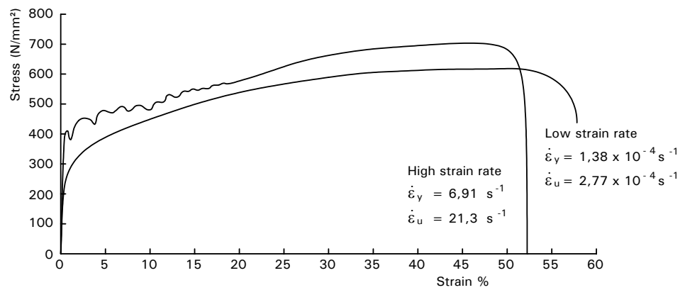
Figure C.3.7 Strain rate effects on grade 1.4404
