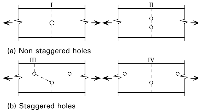
Figure C.4.8 Net section failure modes
