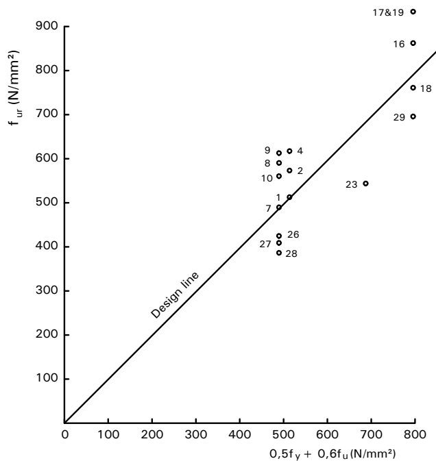
Figure C.6.3 Comparison of f_{ur} design line and experimental data
