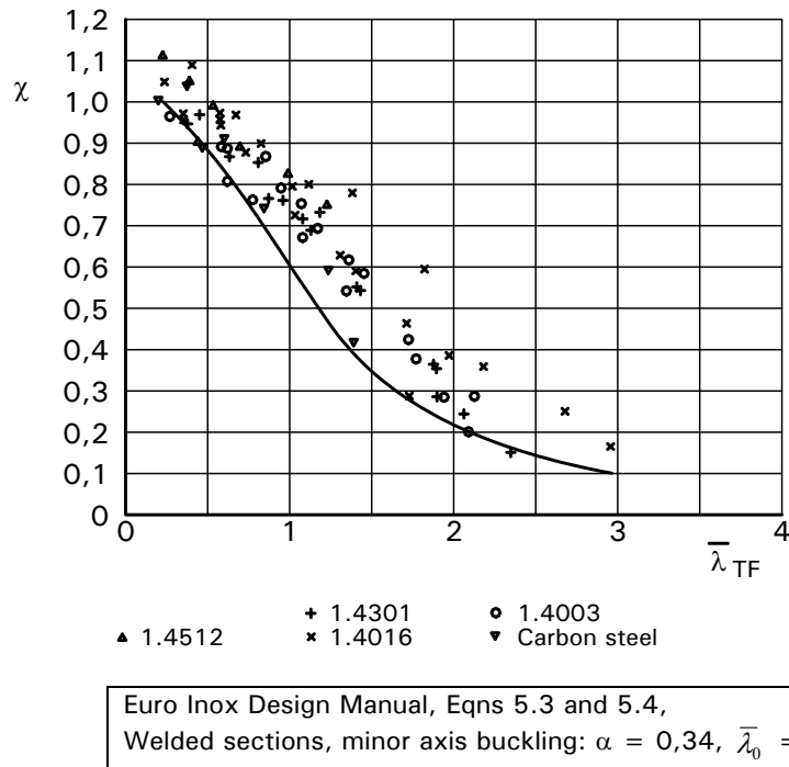
Figure C.5.11 Reduction factor versus non-dimensional slenderness for torsional-flexural buckling
