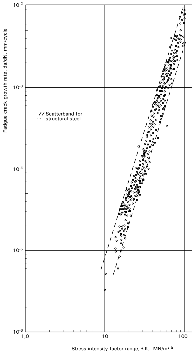
Figure C.8.4 Crack growth rate data for stainless steels in air at temperatures less than 100°C
